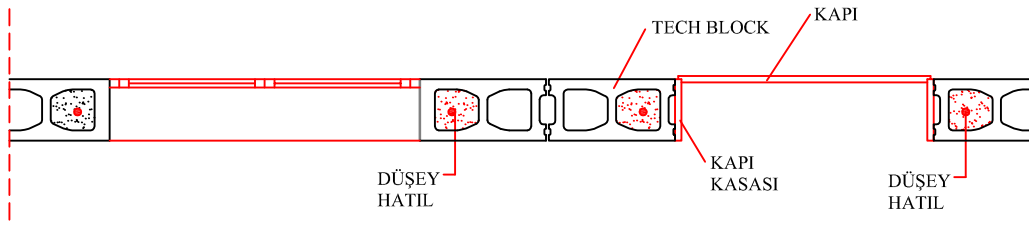
PLAN KESİT
